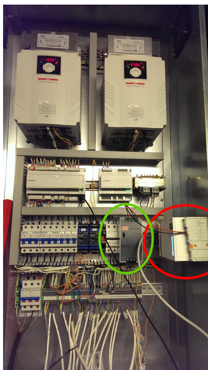
Figure 5 - Equipment added at the ventilation system in the Grundfos Dormitory Lab. The green circle enclose the power supply used to power the embedded PC in the red circle.
