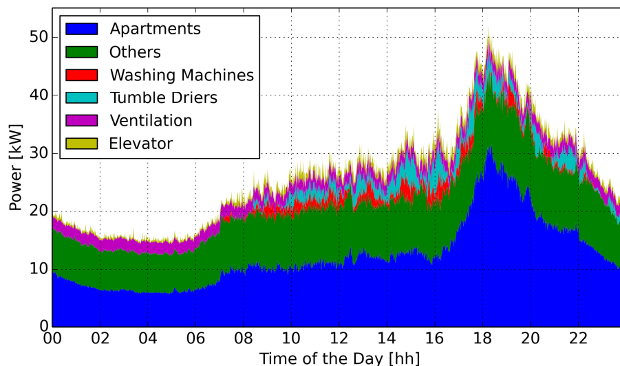
Figure 2 - Averaged power profile of the Grundfos Dormitory Lab from the 18-02-2016 until the 08-03-2016.
