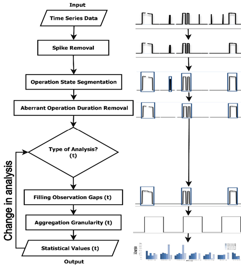
Figure 3: Pre-processing steps
