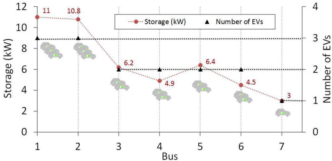
Figure 17. The required storage power and corresponding number of EVs.
