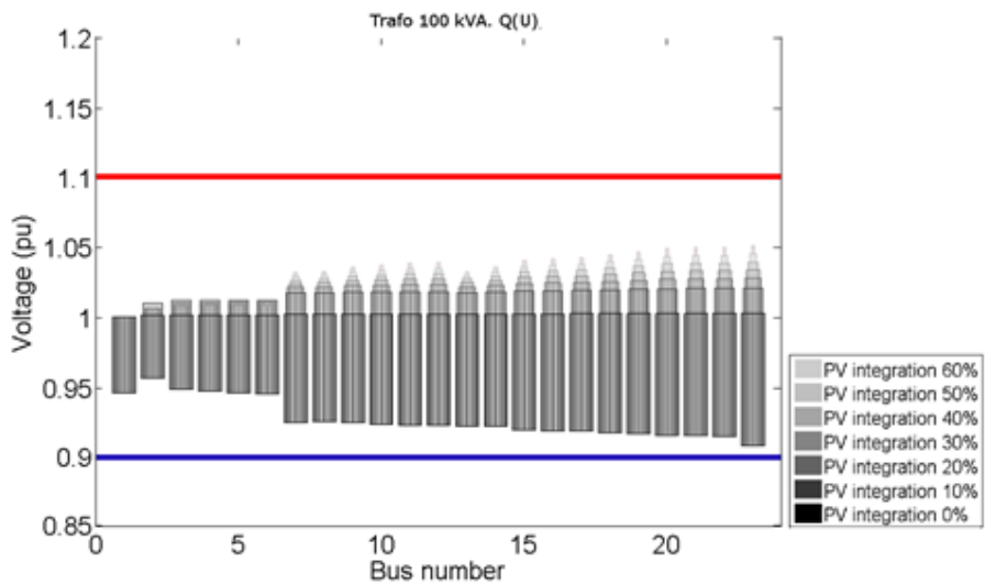
Figure 29. Maximum voltages at different levels of PV penetration along feeder 1 via Q(U).
