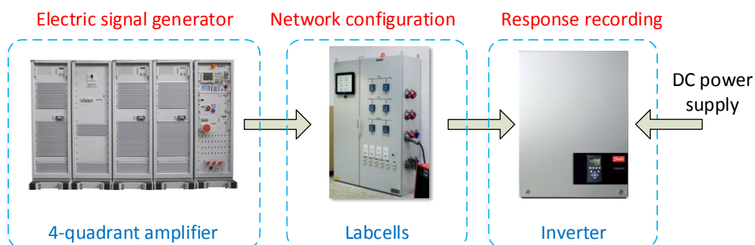
Figure 4. Testing system configuration
