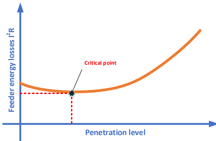
Figure 32. The developing of grid losses with respect to PV penetration level.
