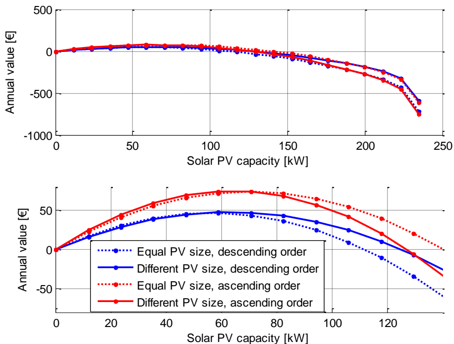
Figure 33: Annual value of solar PV systems in a residential distribution grid, fed by a 100 kVA transformer. The lower plot is a zoom of the upper [21].
