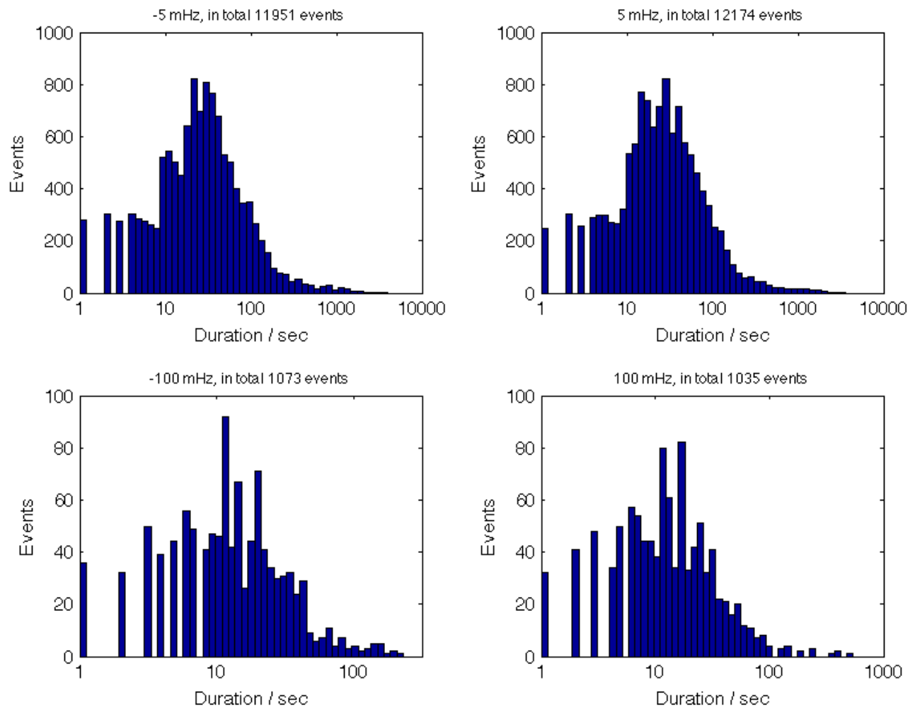
Figure 2.4. Statistical representation of frequency deviations from 50 Hz in DK2 for the period 04-06-10 through 20-06-10. The figure shows the number of events where the deviation exceeded the indicated (above each graph) limits distributed on duration classes. The average frequencies of events are as follows: -5 mHz once every 117 sec, +5mHz every 115 sec, -100 mHz every 22 min, +100 mHz every 23 min.
