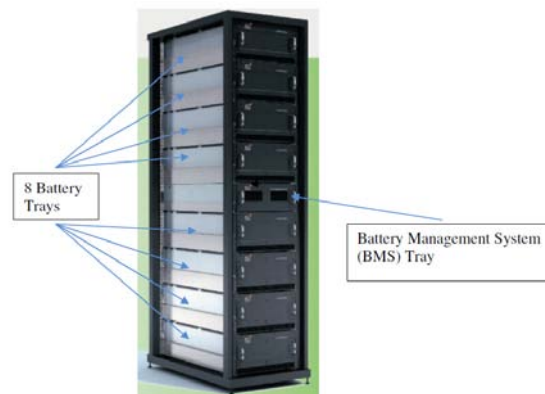
Figure 3.1.6: Suggested rack solution from A123
