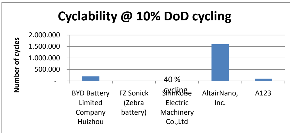
Figure 3.1.17: Number of cycles the battery is capable of with a SOC cycling of 10 %, eg from 70 to 80 % DOD. The data from ShinKobe is at 40 % cycling. The battery is considered exhausted, when the capacity is reduced to 80 % of initial capacity.
