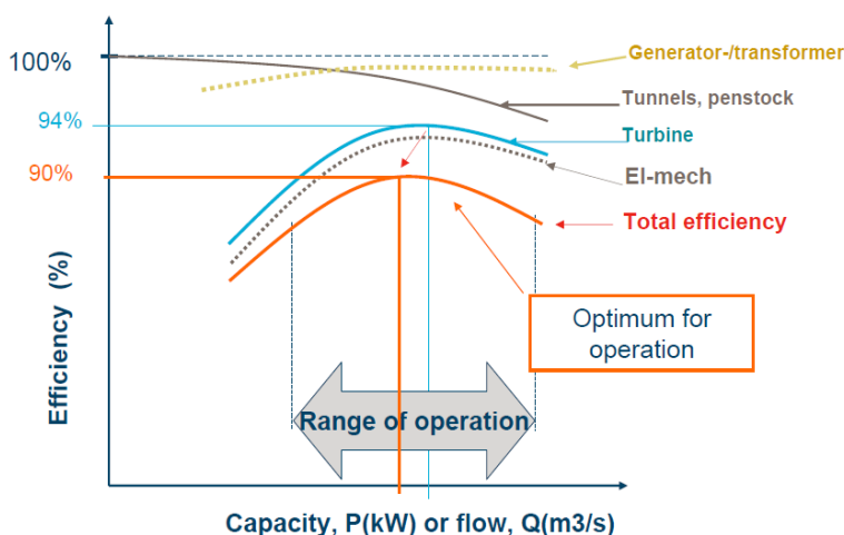
Figure 3.4.3. Efficiency of hydropower plants and break down of losses 28
