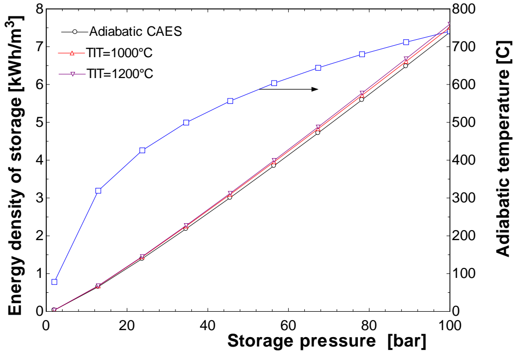
Figure 3.2.6 CAES energy storage density
