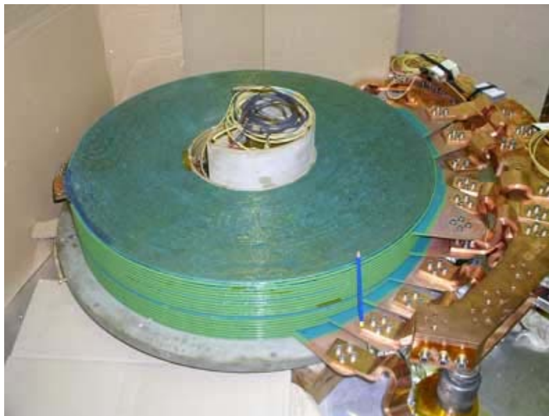
Figure 3.6.1. Photo of a laboratory scale SMES at the NEEL, CNRS, France 49 . The device is based on BiSrCaCuO and is able to store approx 800 kJ (about 0.2 kWh). Coil dimensions are: external diameter 814 mm and height 222 mm.
