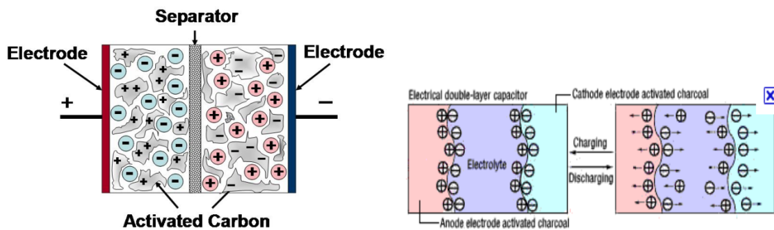
Figure 3.5.1. The left part 33 shows the construction of a supercapacitor. The shown electrodes consist of finely structured (nanostructured) carbon which gives a large electrode surface area and accordingly a large double layer as well as short diffusion distances for the migrating charged particles. The right part 34 of the figure illustrates the mechanisms of charging and discharging. During charging the charged particles are attracted to the electrode surfaces and thereby form the double layer. During discharge the particles mix randomly.
