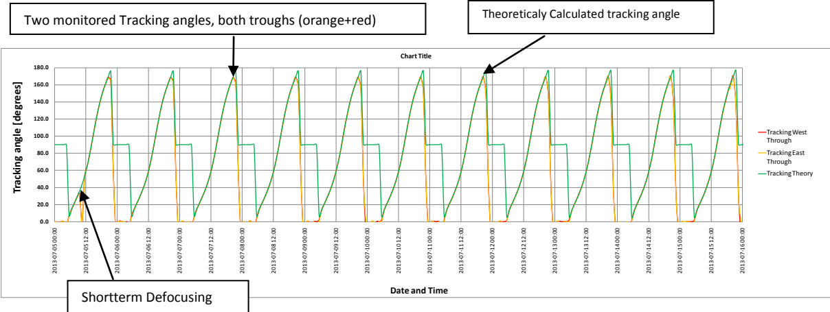
Figure 7. Check of tracking accuracy for both troughs and comparison to theoretical tracking angle based on time of day/year and solar position and geometry using the theory in ref [5] and [6]. The match is almost perfect within 0.5^\circ , except the first day when some maintenance was done. Same period as for the performance in Figure 6.
